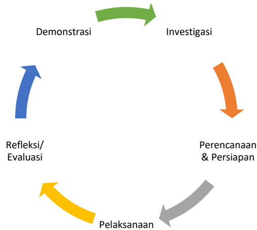
Gambar 1. Diagram Service-Learning
